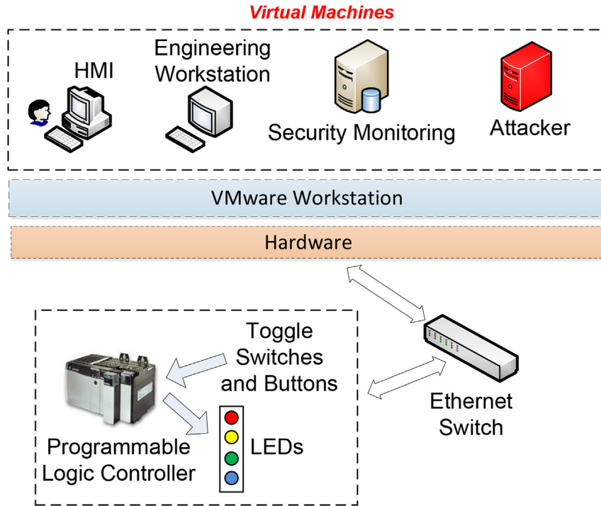
Fig. 6. The experimental setup for the evaluation of Cutter.
