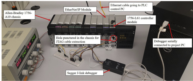
Fig. 11. PLC experimental setup for the case study.
