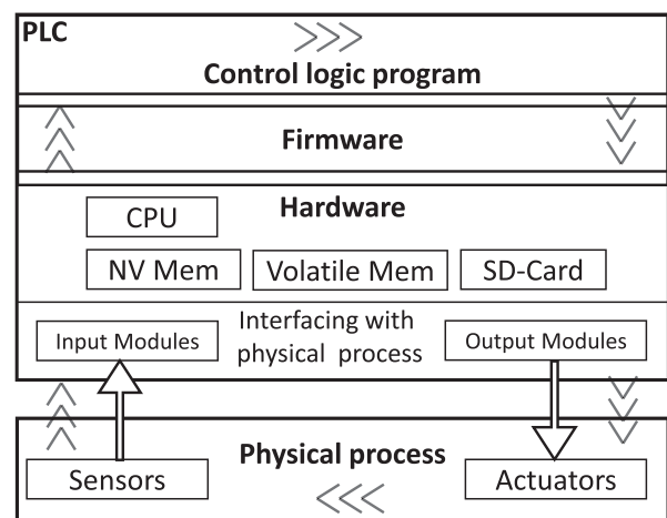
Fig. 1. PLC architecture.
